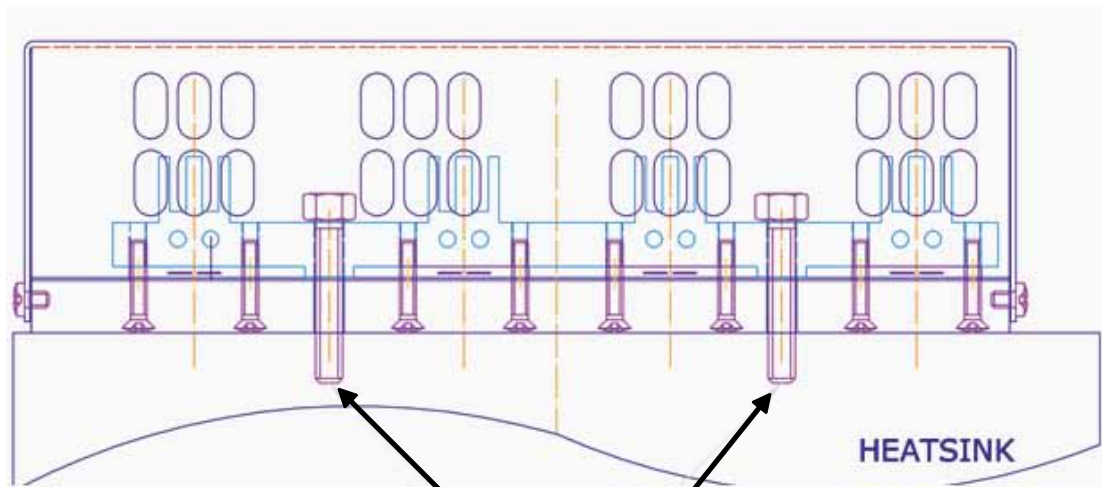
M5 X 25 SCREWS (7 PLACES)
