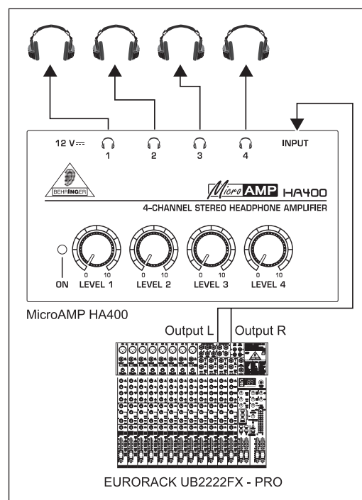
Example: HA400 wiring
